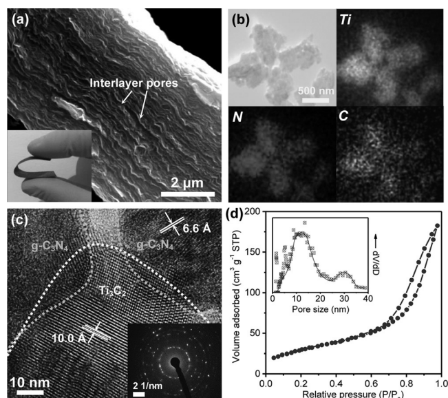
Figure 2. a) SEM, inset in panel a) optical, b) EDS elemental mapping, c) HRTEM images, and inset in panel c) SAED pattern of TCCN. d) \text{N}_2 adsorption isotherm, and inset in panel d) the corresponding differential pore size distribution for TCCN.
