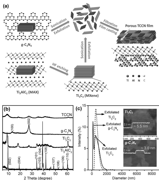
Figure 1. a) Fabrication of the porous TCCN film. b) XRD patterns of \text{Ti}_3\text{AlC}_2 , \text{Ti}_3\text{C}_2 , \text{g-C}_3\text{N}_4 , and TCCN. c) Particle size distributions of the \text{Ti}_3\text{C}_2 dispersion and the mixed dispersion of \text{Ti}_3\text{C}_2 and \text{g-C}_3\text{N}_4 after exfoliation. inset in panel c) AFM images of exfoliated \text{Ti}_3\text{C}_2 and \text{g-C}_3\text{N}_4 nanosheets.
